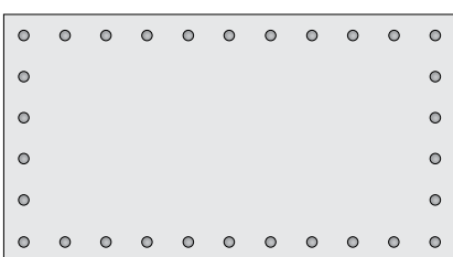
MH09.O 1865x1020x65mm
